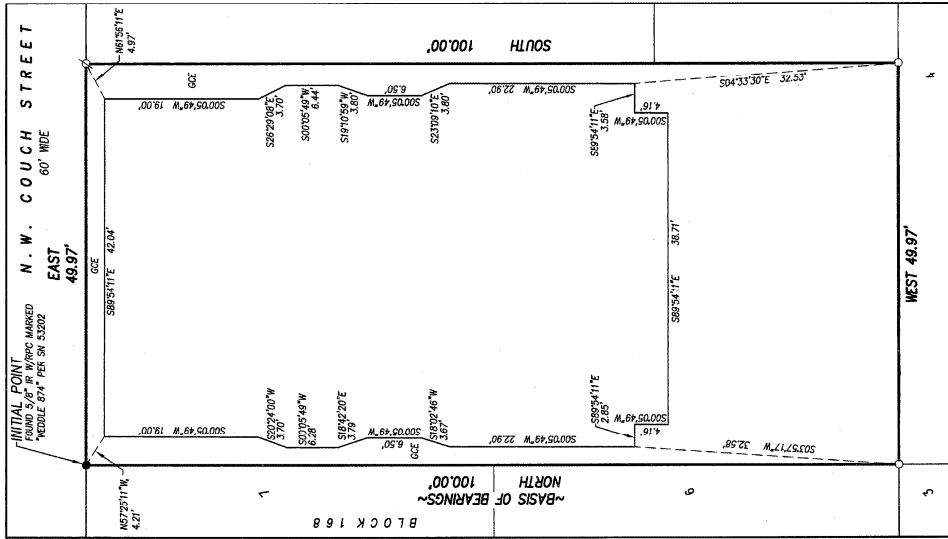
BASEMENT RELATIVE TO PLAT BOUNDARY
