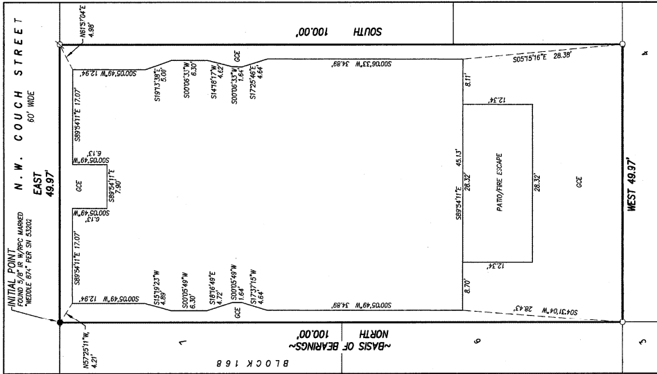
FIRST FLOOR RELATIVE TO PLAT BOUNDARY
